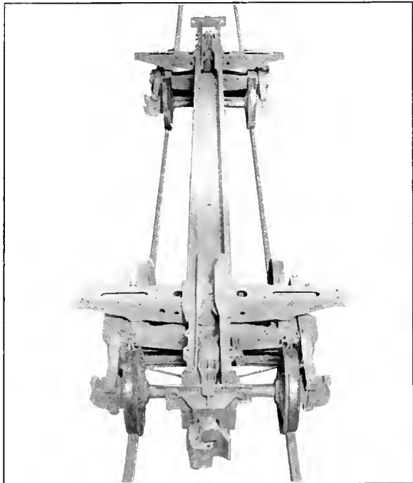
Underframe Ready for Application of Car Body
